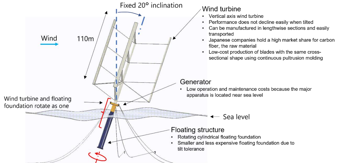
Artist's concept of a floating axis wind turbine (5MW demonstrator) (Courtesy of Albatross Technology Inc.)
